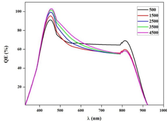
Figure 5. Quantum efficiency of ZnO/CdS/CdTe solar cells with variations in thickness of CdTe
