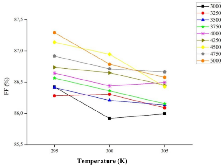
Figure 6. Effect of device temperature change on FF
