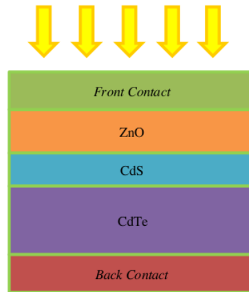
15 Figure 1. Schematic of a ZnO / CdS / CdTe solar cell layer
