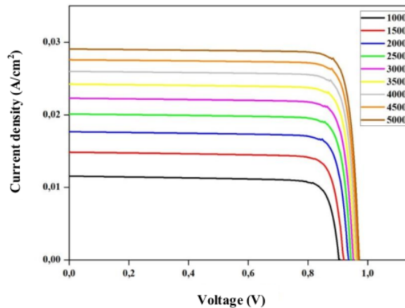
Figure 2. Graph of relationship of current density to voltage on ZnO/CdS/CdTe solar cells
