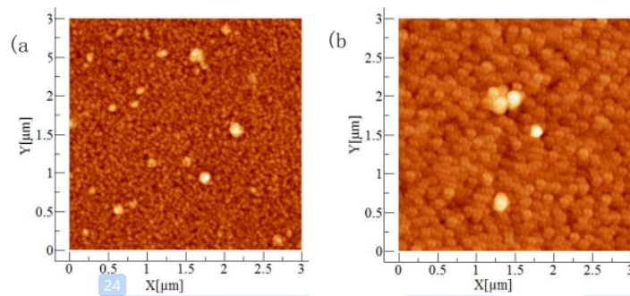
Figure 3. AFM images of AZO (2 at% Al) thin films growth with the sputtering power of (a) 30 Watt and (b) 40 Watt.
