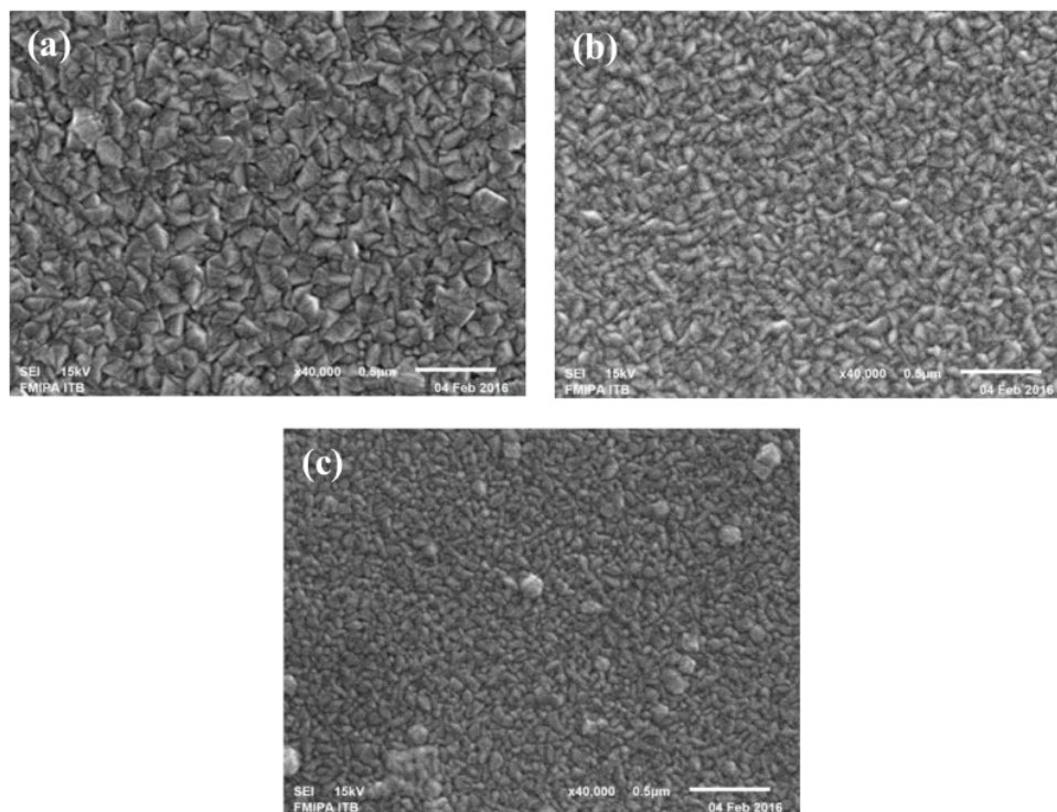
8 Figure 1. SEM images of ZnO:Ga thin films with different annealing temperatures: (a) 300 °C, (b) 350 °C, and (c) 400 °C.
