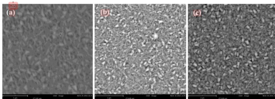
Figure 2. SEM images of ZnO:Al thin films with Oxygen pressure at annealing process : a) 0 mTorr, b) 50 mTorr, and c) 100 mTorr.
