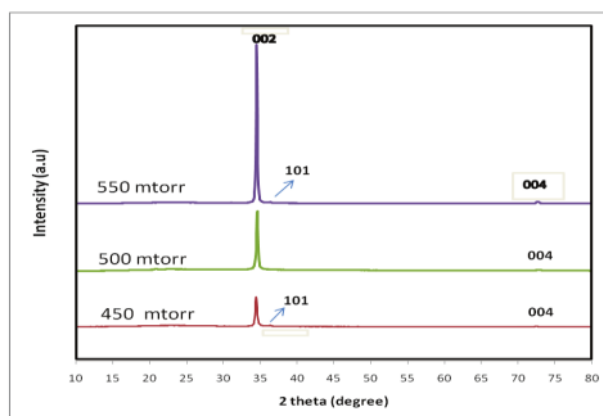
FIGURE 1. X-ray diffraction patterns of ZnO:Ga films deposited at different argon pressures.
