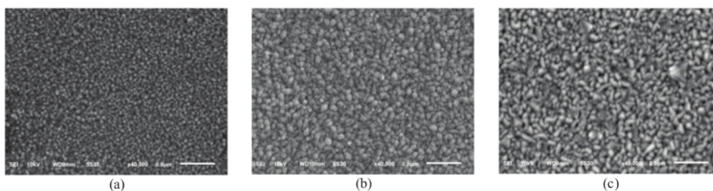
FIGURE 2. SEM morphologies of ZnO:Ga thin films deposited with different pressures: (a) 450 mtorr, (b) 500 mtorr, and (c) 550 mtorr
