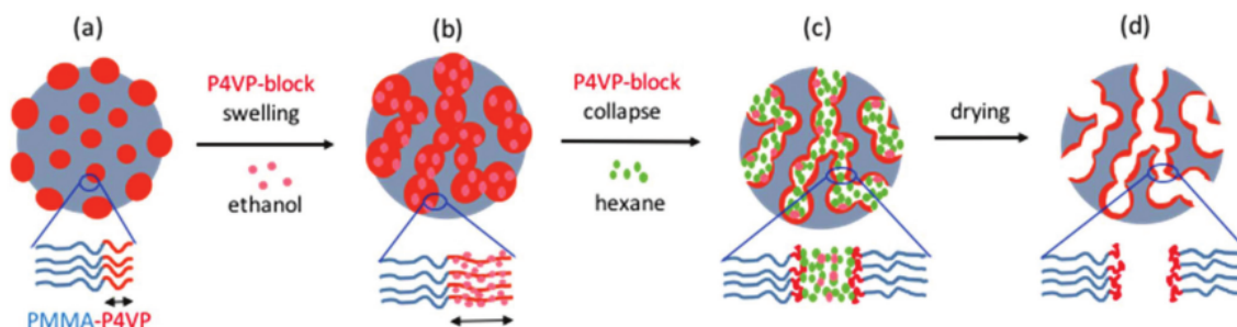
Scheme 1 Schematic demonstration of pore generation through BCP microparticles via selective solvent swelling induced order-to-order morphology transition and then morphology fixation by fast de-swelling.
