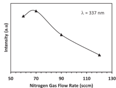
FIG. 2. Dependence of the emission intensity of nitrogen plasma for the 337-nm peak on the flow rate of nitrogen gas at a substrate temperature of 650 °C. Lines between points are only included as guides to the eye. Intensity reaches its maximum at a nitrogen flow rate of 70 SCCM.
