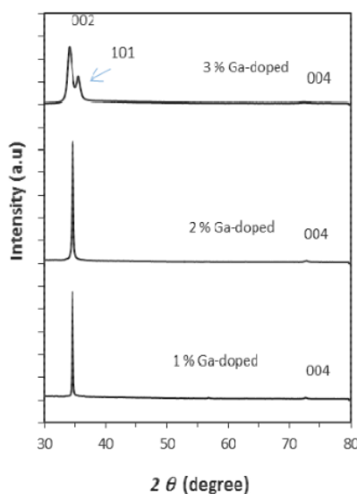
33 Fig. 1. X-ray diffraction patterns for ZnO:Ga thin films deposited at different Ga-doped concentration
