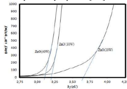
Figure 4. Relation (ah\gamma)^2 with the bandgap energy (h\gamma) ZnO films deposited at room temperature with a plasma power of 20, 30, 40W.
