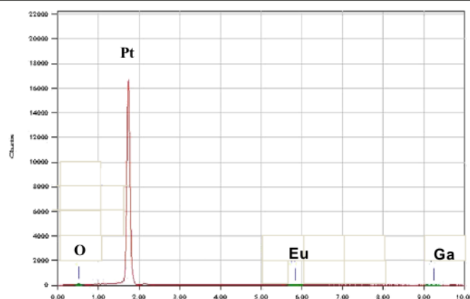
Figure 1 EDX spectra of \text{Ga}_2\text{O}_3\text{:Eu} (5%) thin film.
