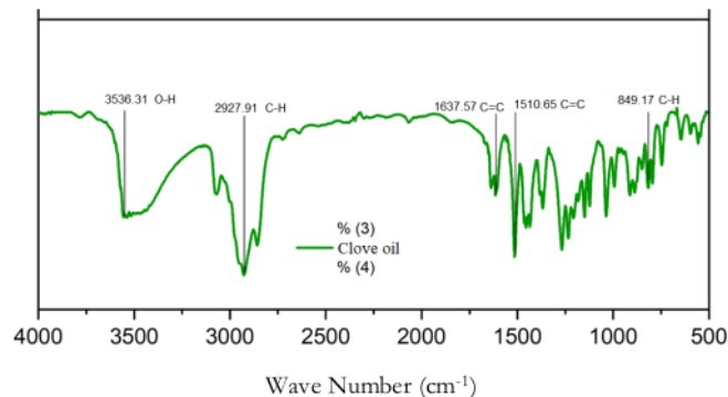
Figure 3. Clove oil IR spectrum ( \text{cm}^{-1} )
