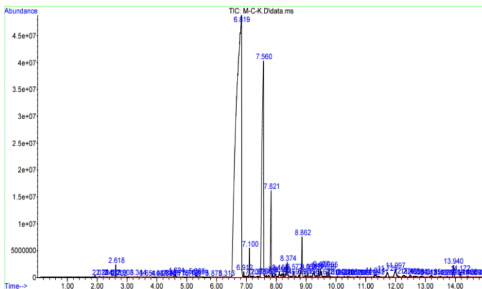
Figure 4. Clove oil GC-MS Chromatogram
