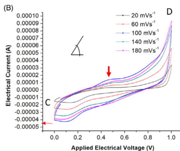
FIGURE 4 Cyclic voltammograms of anthocyanins in various scan rates: A, without microwave irradiated and B, with microwave irradiated [Colour figure can be viewed at wileyonlinelibrary.com ]
