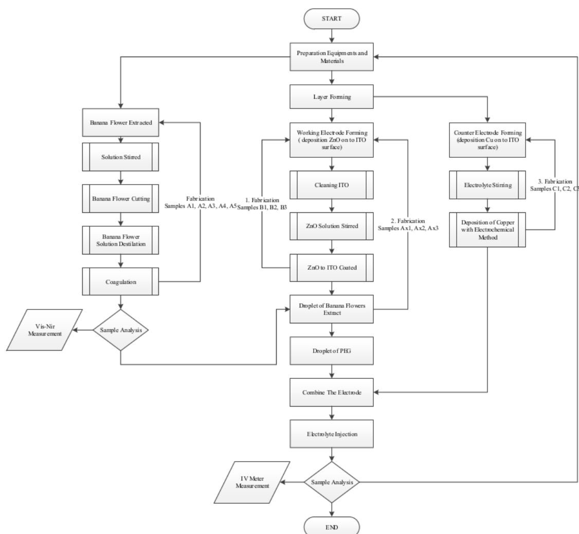
Fig. 2. Flow-chart of DSSC fabrication technology.
