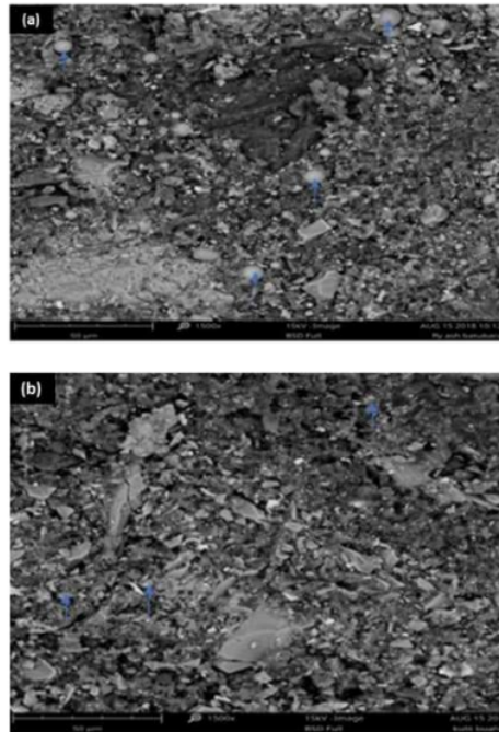
Figure 4. SEM images in magnification of 1500X of brake composite containing: (a) Mahogany rind carbon and (b) coal fly ash.
