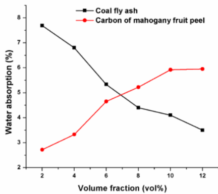
Figure 3. Water absorption for each composite brake linings on the different volume fraction (37.4) Mahogany rind carbon and (b) coal fly ash.
