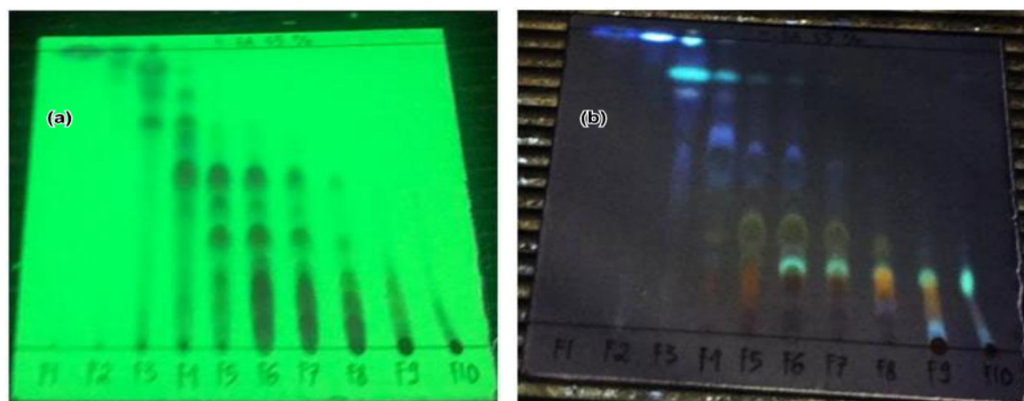
Fig. 1. Thin-layer chromatography (TLC) profile of subfractions 1-10 of sappan wood ( Caesalpinia sappan L.) extract resulted from vacuum liquid chromatography (VLC) using (a) 366 mm and (b) 254 mm UV lamp
