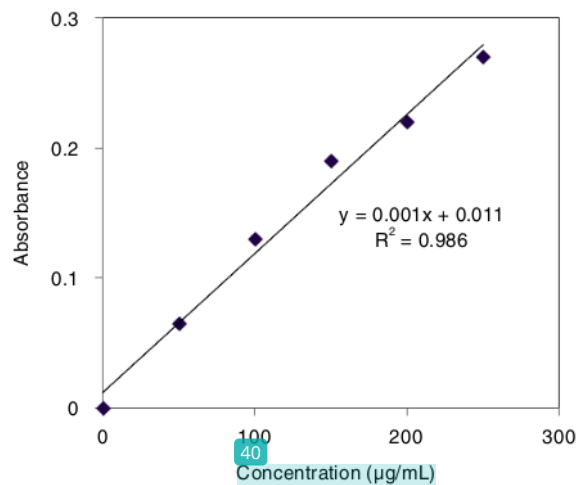
Fig. 2. Calibration curve of gallic acid at a maximum wavelength of 765 nm
