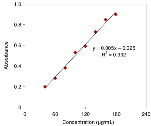
Fig. 3. Quercetin calibration curve at a maximum wavelength of 425 nm
