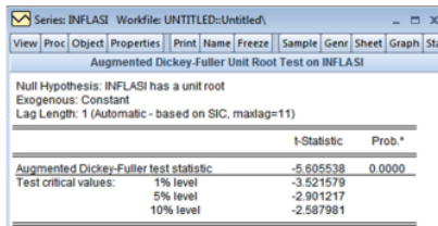
Figure 7. Unit Root Test Results
