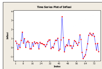
Figure 2. Time Series Plot for Inflation
