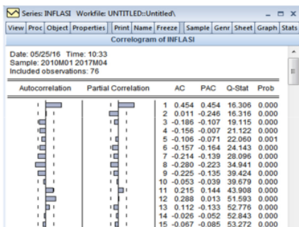
Figure 6. Correlogram of Data
