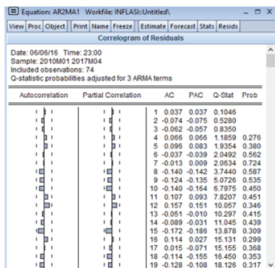
Figure 11. Correlogram of residual ARIMA(2,0,1) or ARMA(2,1)
