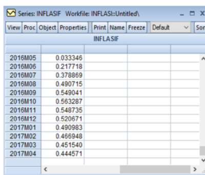
Figure 13. Inflation Data Forecast Results in Semarang district
