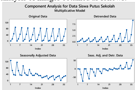
Figure 7 Trend Analysis Models Multiplicative
