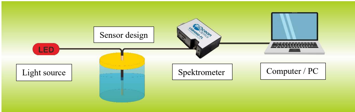
Figure 3. Characterization setup
