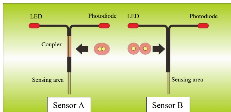
Figure 1. Viscosity sensor based on POF
