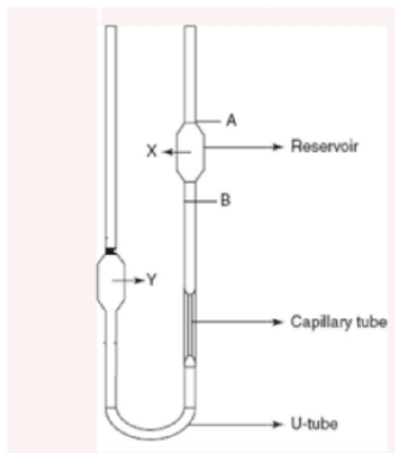
Gambar 1 viskometer Ostwald
