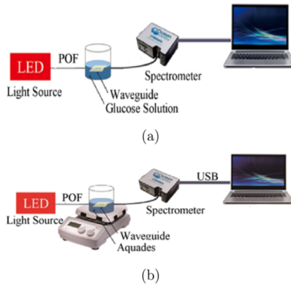
Fig. 2. Characterization set up for RI response (a) and temperature response (b).
