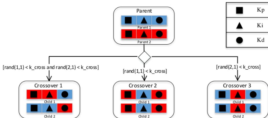
Figure 4. Chromosome's crossover of PID parameters
