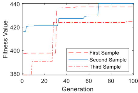
Figure 5. Three trials with generation size 100
