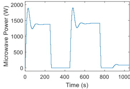
Figure 9. Generated PID control signal
