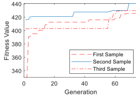
Figure 6. Trials with different population
