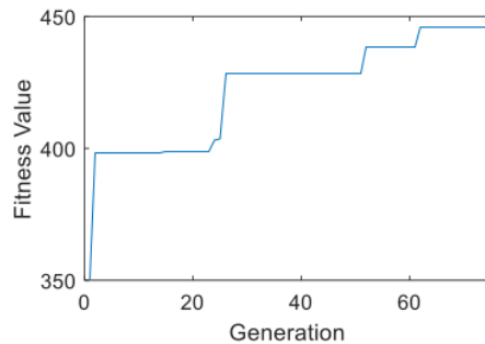
Figure 7. Best fitness value of each generation
