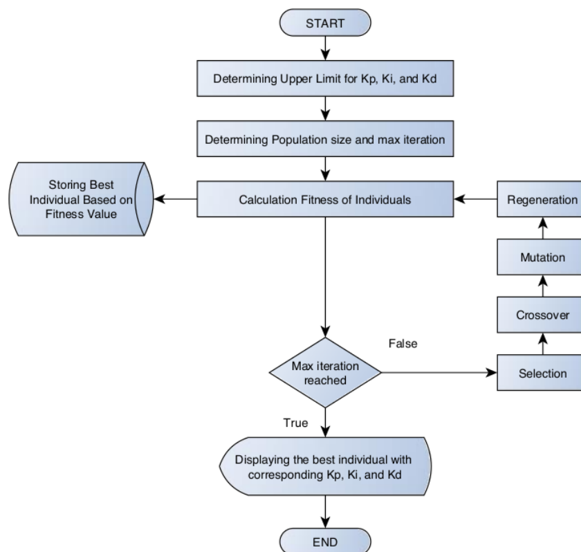
Figure 3. Flowchart of GA-based tuning for PID controller.
