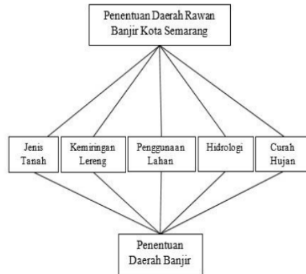
Fig 2. Analytical Process
