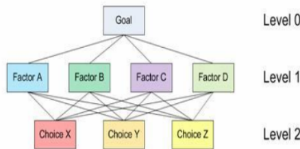
Fig. 1 Analytical Hierarchy Process Concept
