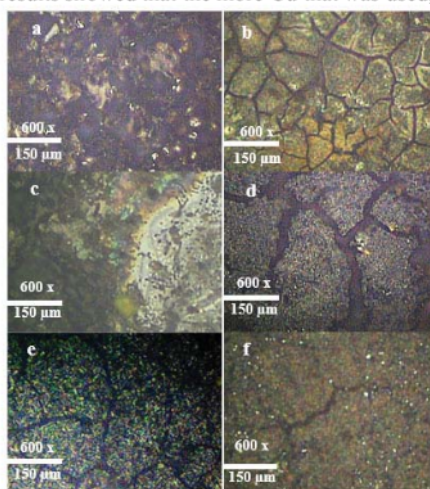
FIGURE 4. CCD (a) SLG A film, (b) ITO A film, (c) SLG B film, (d) ITO A film, (e) SLG C film, (f) ITO C film.
