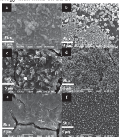
FIGURE 5. SEM (a) SLG A film, (b) ITO A film, (c) SLG B film, (d) ITO A film, (e) SLG C film, (f) ITO C film.
