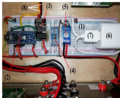
Figure 2. The microcontroller components
