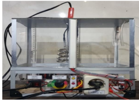
Figure 4. The rear IoT based learning media
