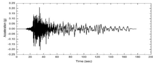
Figure 4. Base input motion.
