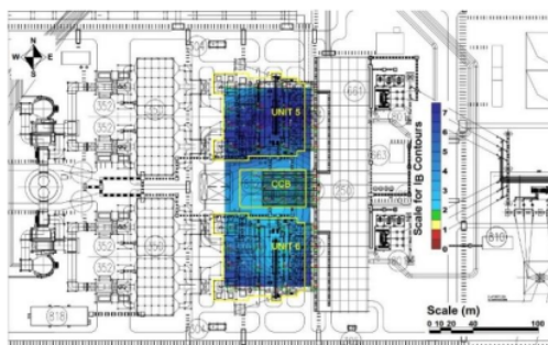
Figure 2. I_B contours for post-liquefaction in wet season.
