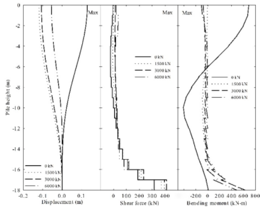
Fig. 8. Maximum pile response profiles during the shaking.
