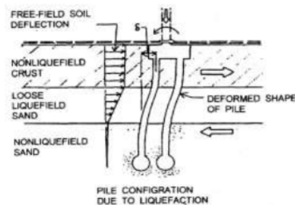
Fig. 1. Potential failure mode of piles due to seismic loading and soil liquefaction (Finn and Thavaraj, 2001).
