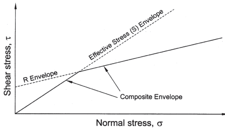
FIGURE 3. Composite of Shear Strength Envelope 7
