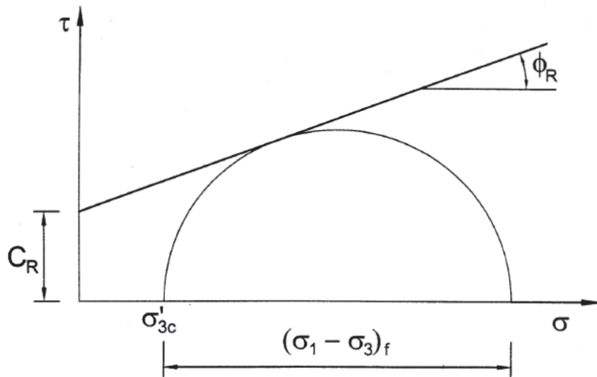
FIGURE 1. Mohr Coulomb Diagram 7
