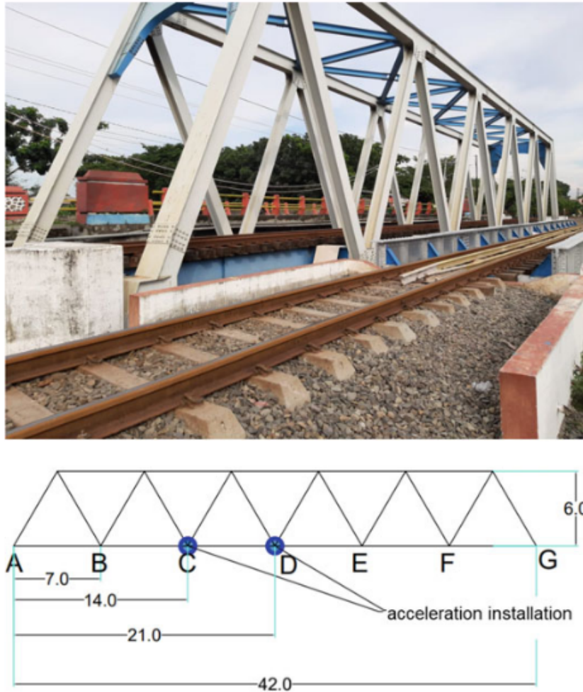
Fig. 1 Railway bridge and acceleration installation
