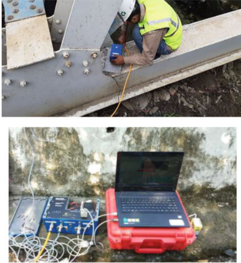
Fig. 2 Sensor installation and a set of measurements
