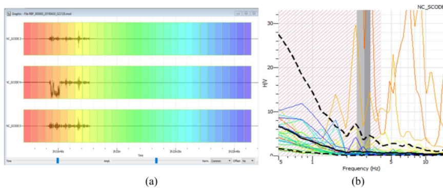
FIGURE 8. (a) Display of the vibration signal in the Geopsy software; (b) Graph of the relationship of natural frequencies with H / V
