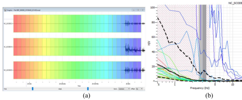
FIGURE 7. (a) Display of the vibration signal in the Geopsy software; (b) Graph of the relationship of natural frequencies with H / V
