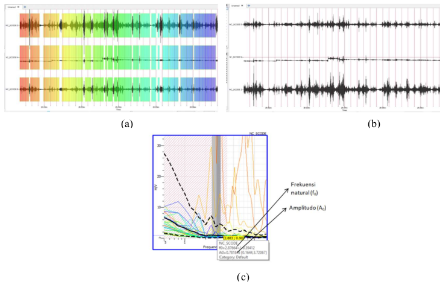
FIGURE 2. Display in the Geopsy software (a) Graph of vibration acceleration; (b) Graph of vibration acceleration after signal selection; (c) Graph of the relationship of natural frequencies and H / V.
