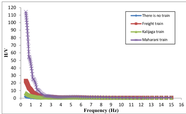
FIGURE 10. Graph of the relationship of natural frequencies with H/V in terms of the type of train passing the railway
