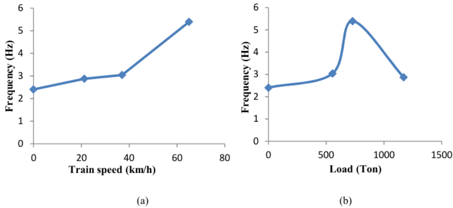
FIGURE 11. (a) The graph of natural frequency and train speed; (b) The graph of natural frequency and loads.
