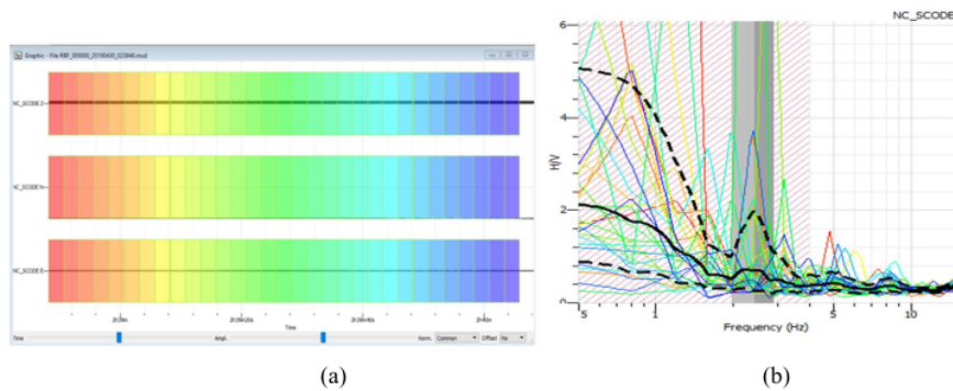
FIGURE 6. (a) Display of the vibration signal in the Geopsy software; (b) Graph of the relationship of natural frequencies with H / V
