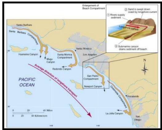
FIGURE 4. Illustration of Longshore Sediment at Pacific Coastal [3]
