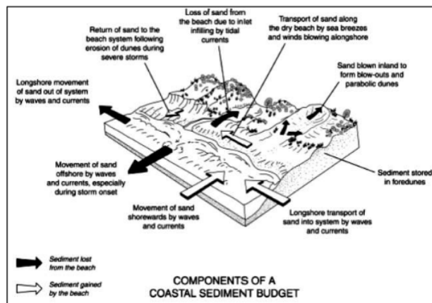
FIGURE 3. Mechanism of Coastal Sediment Budget [2]
