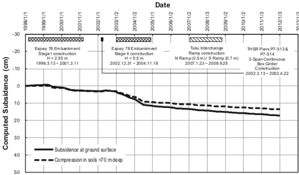
Fig. 14. Influence of Expyw 78 embankment loading on compression of soils at the intersection of THSR and Expyw 78 between 01/1998 and 12/2011.
