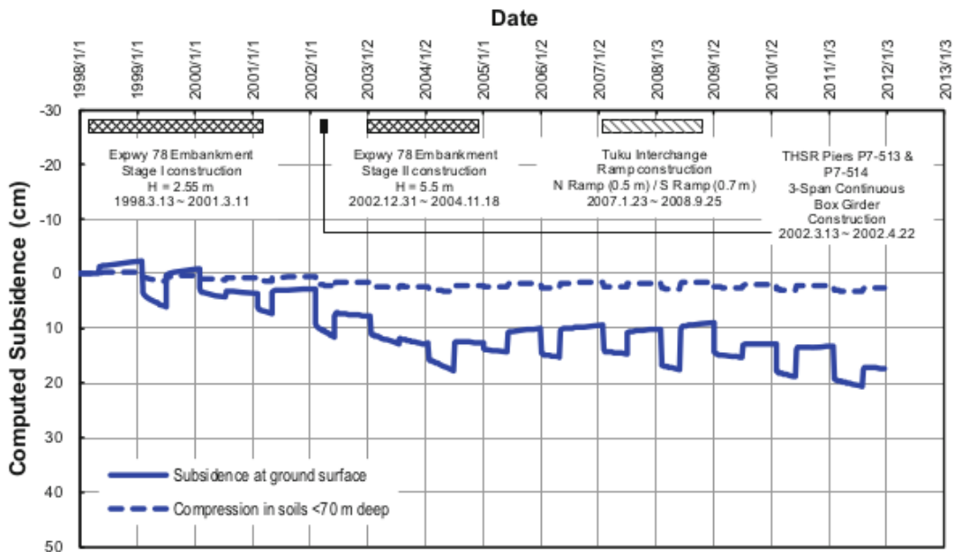
Fig. 16. Influence of groundwater level fluctuation on compression of soils at the intersection of THSR and Expwy 78 between 01/1998 and 12/2011.
