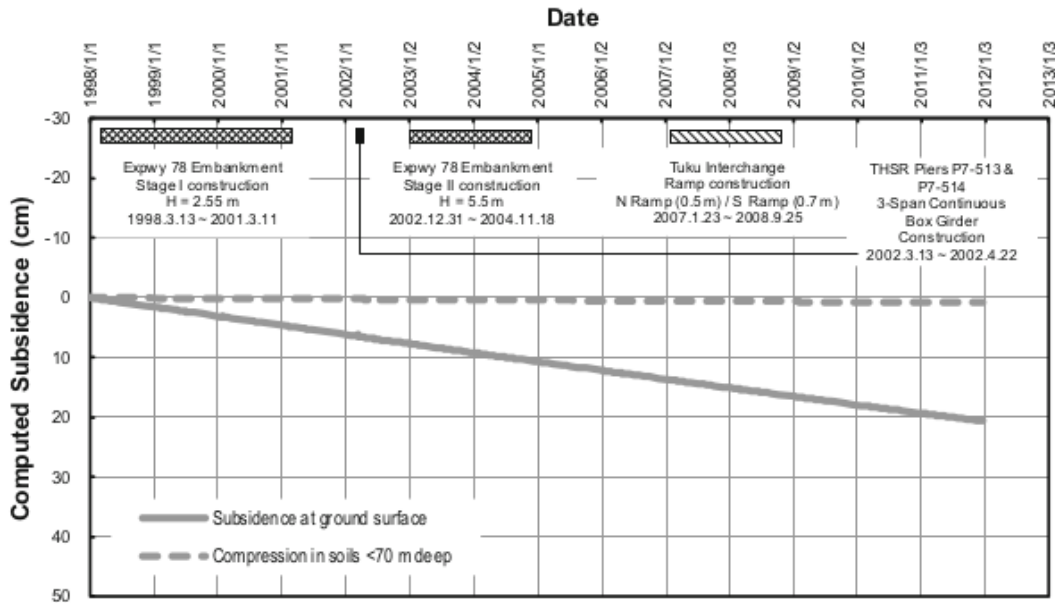
Fig. 12. Influence of soil creeping on compression of soils at the intersection of THSR and Expwy 78 between 01/1998 and 12/2011.
