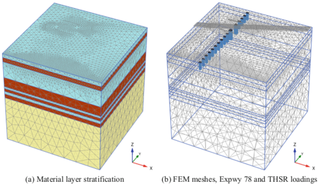
Fig. 10. FEM model adopted in numerical simulations.
