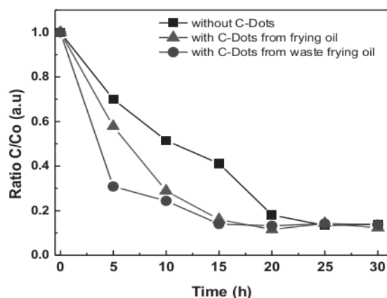
FIGURE 3. Degradation Intensity of the Methylene Blue Absorption.
