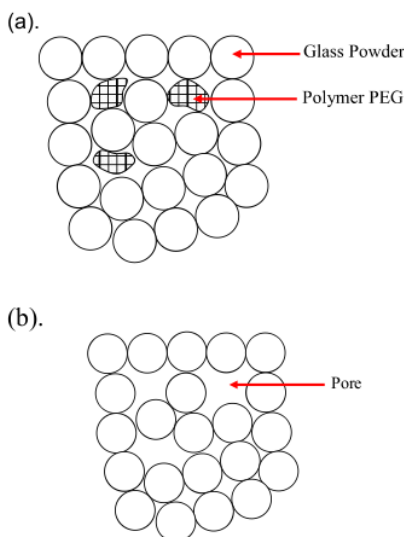
Figure 1. Illustration of (a) composite before the heating process and (b) pores formed after the heating process.
