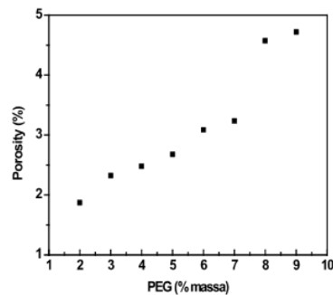
Figure 3. The distribution of porosity value of porous composite one layer.
