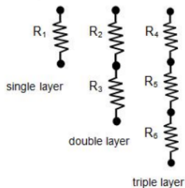
Figure 8. Illustration of a resistance model of fluid through the multilayer porous composite medium.
