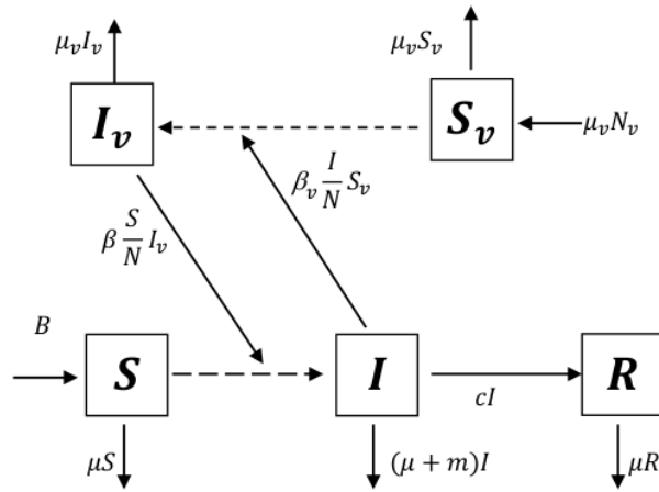
Figure 1. Transfer diagram of Zika epidemic
