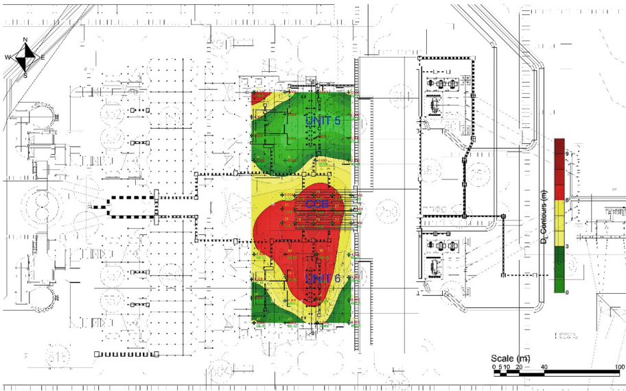
Fig. 7. D_L contours for post-liquefaction in wet season.
