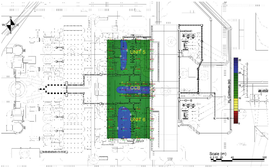
Fig. 8. H_C contours for post-liquefaction in wet season
