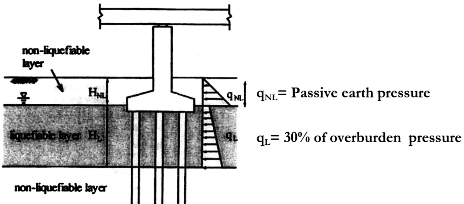
Fig. 2. The idealization for seismic design (JRA 1996)
