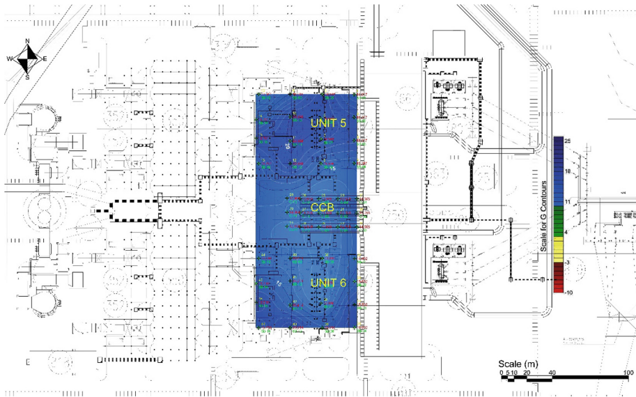
Fig. 9. G contours for post-liquefaction in wet season.
