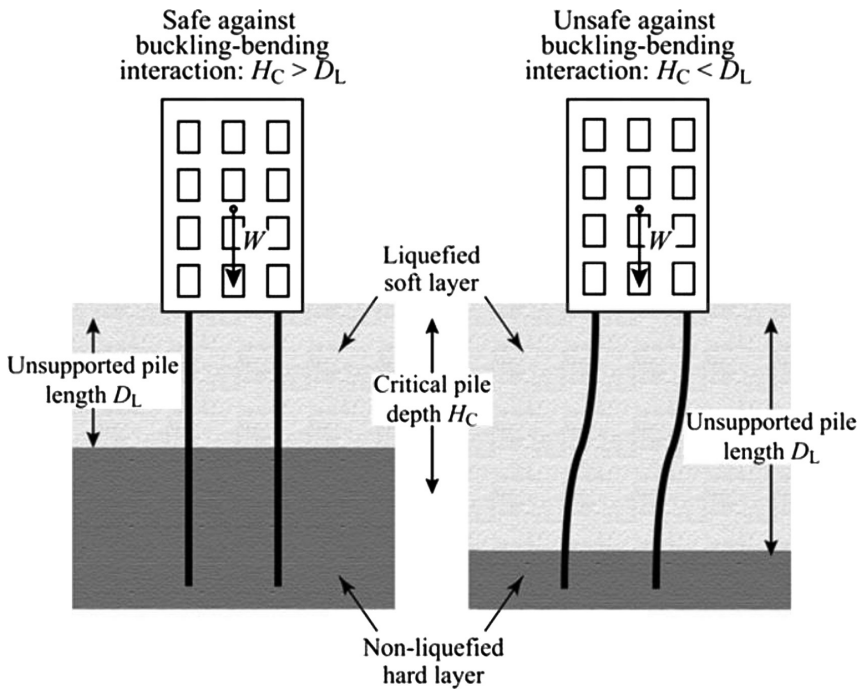
Fig. 5. Concept of critical length ( H_C ) and unsupported length ( D_L ), Bhattacharya (2015).
