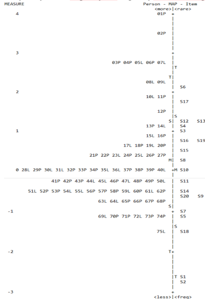
Figure 2. Wright map
