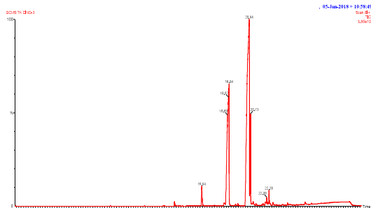
Figure 3. Biodiesel from WCO Chromatogram.
