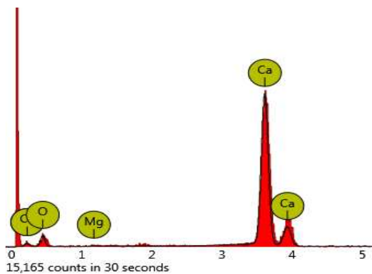
Figure 1. EDX Analysis of Eggshell CaO Catalyst.
