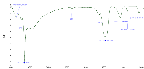
Figure 6. FTIR Analysis of ZnO/CaO 6% Catalyst.
