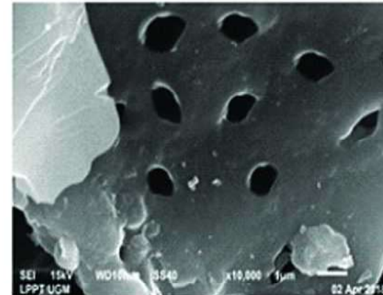
SEM micrograph of Teak sawdust based activated Carbon
