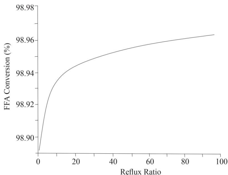
Figure 2. The Effect of Reflux Ratio on the FFA Conversion
