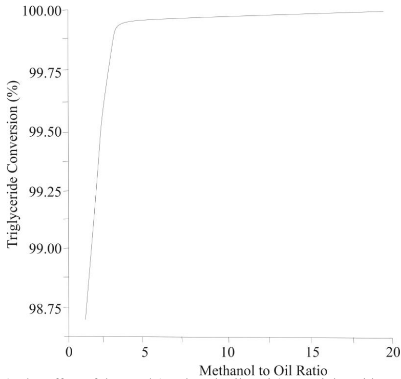
Figure 6. The Effect of the Feed (Methanol-Oil Ratio) on Triglyceride Conversion
