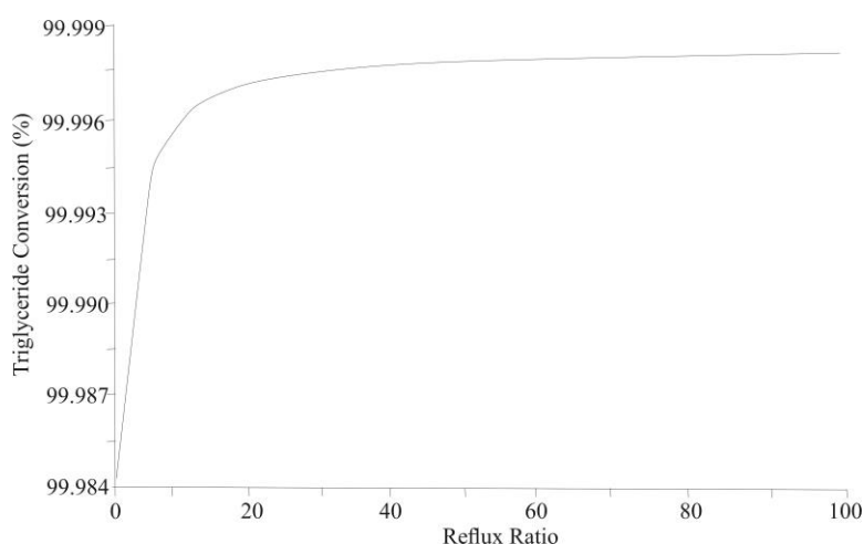
Figure 5. The Effect of Reflux Ratio on Triglyceride Conversion
