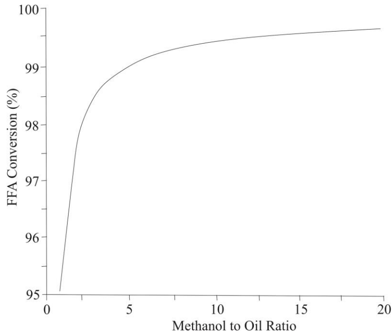
Figure 3. The Effect of the Methanol to Oil Ratio on the FFA Conversion
