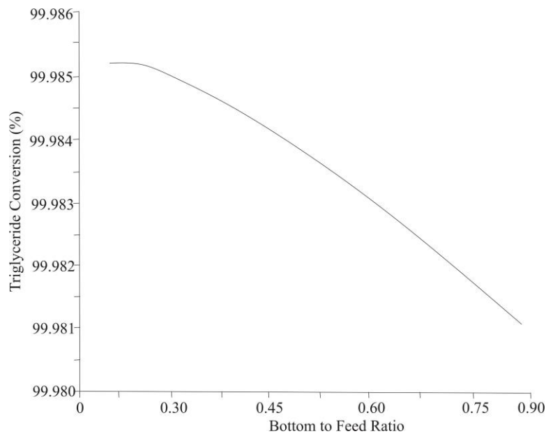
Figure 7. The Effect of the Bottom to Feed Ratio on the Triglyceride Conversion
