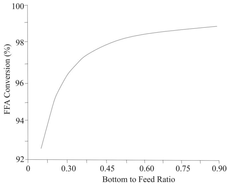
Figure 4. The Effect of Bottom to Feed Ratio on the FFA Conversion
