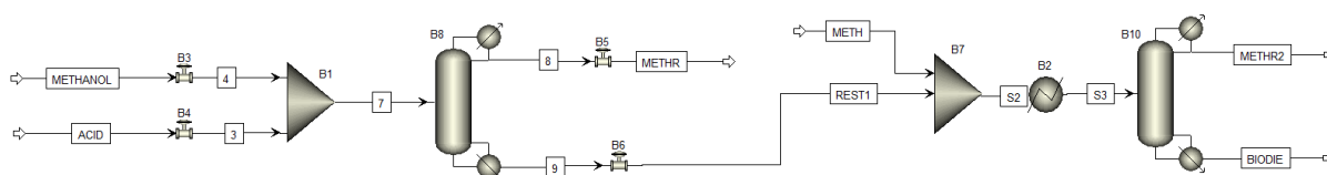
Figure 1. Steady State Aspen Plus v10.0 Simulation Flowsheet of the IDC-RC of Biodiesel Production
