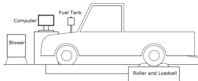
Figure 1. Schematic experimental setup for engine performance test.
