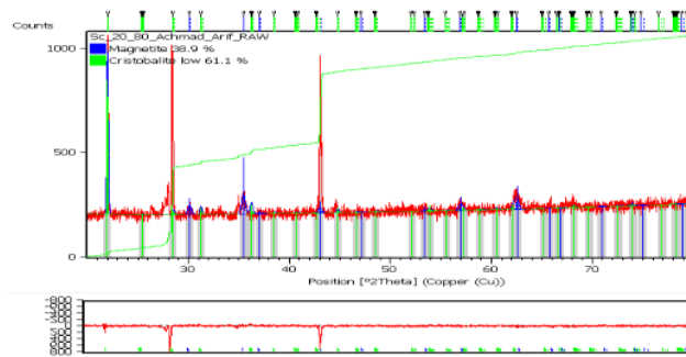
19 Figure 3. The results of quantitative analysis of two main compounds in iron sand.
