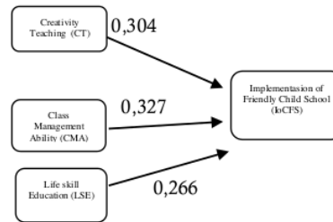
Figure 1. Regression Analysis
