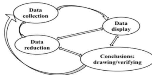
Figure 1. data analysis
