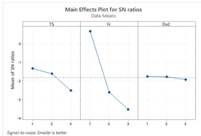
Figure 5. S/N Ratio plot on machining time
