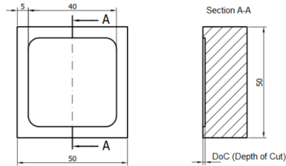
Figure 1. Geometry specimen
