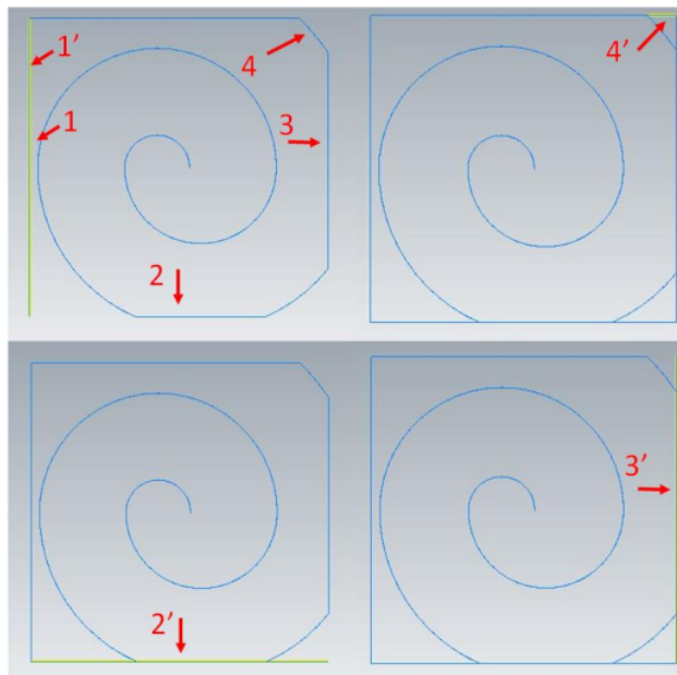
Figure 4. Path repetition on true spiral toolpath
