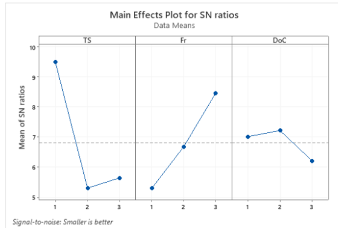
Figure 3. S/N ratio plot on surface roughness
