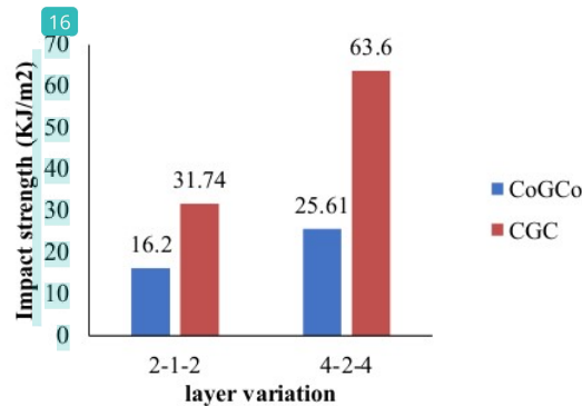
Figure 2. Impact strength
