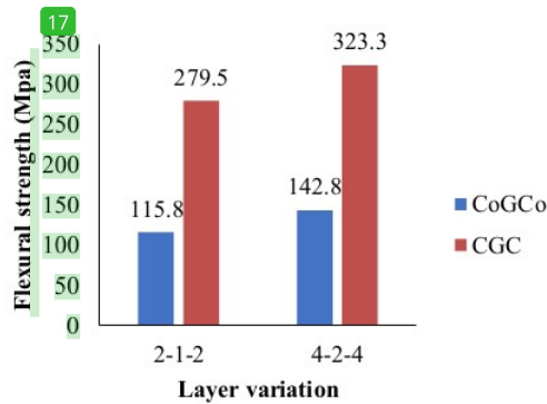
Figure 1. Flexural strength
