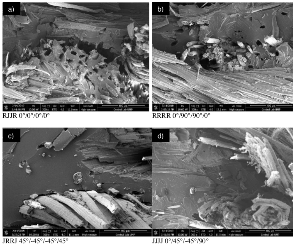
Figure 7. Fracture surface of tensile test.
