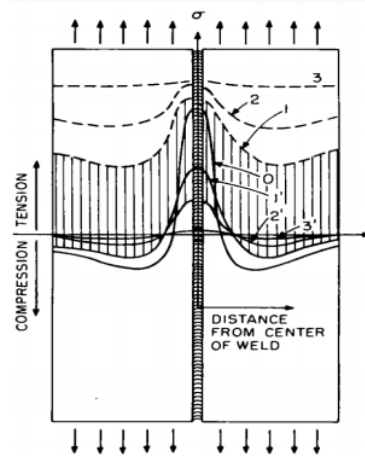
Figure 8. Schematics distributions of stresses on a butt weld when uniform tensile load are applied and of residual stresses after the loads are released [17]
