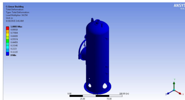
Figure 10. Buckling simulation results
