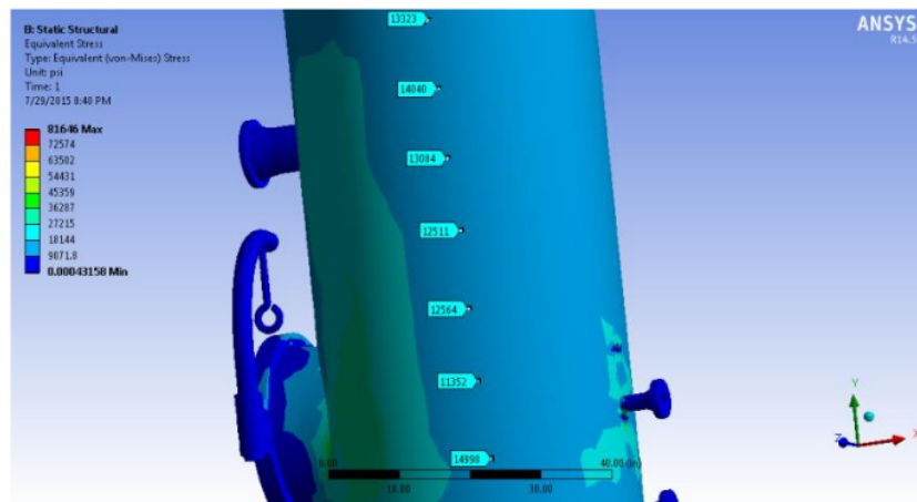
Figure 2. Results of simulation
