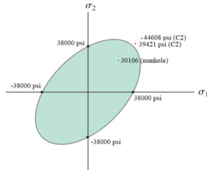
Figure 5. Validation result using theory of distortion energy
