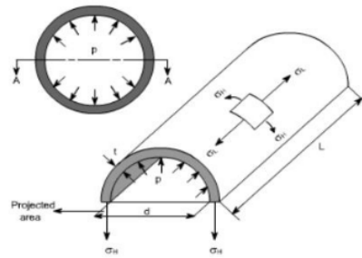
Figure 6. Hoop stress and longitudinal stress [13]
