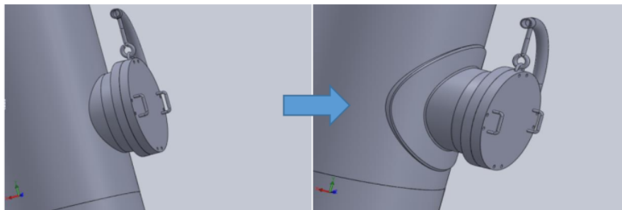
Figure 12. Refinement at manhole area
