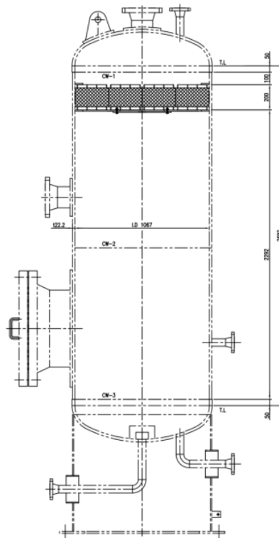
Figure 1. Vertical pressure vessel without the saddle
