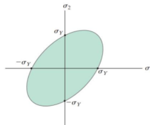
Figure 4. Maximum distortion energy theory [5]
