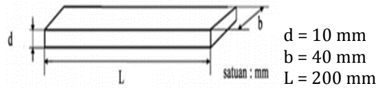
Gambar 1. Spesimen uji bending standar ASTM D790 – 02.
