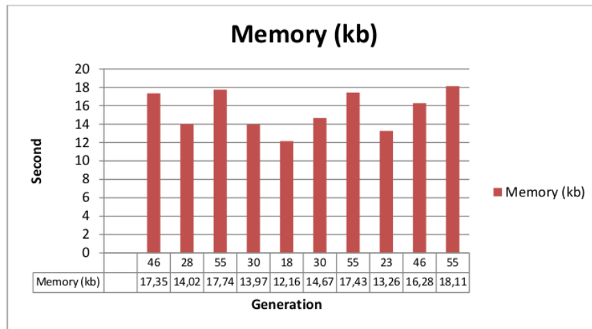
Figure 3. Memory genetic algorithm
