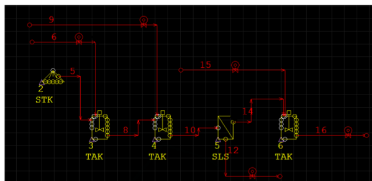
Figure 1: Flowsheet of Thorium Separation Process.
