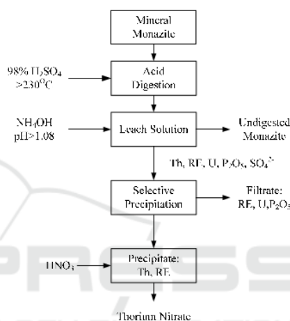
Figure 1: Flow diagram process for monazite digestion and thorium recovery (Al-Areqi, 2016).
